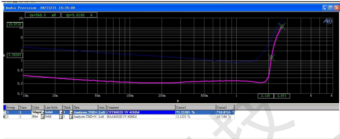
CST8002D THD vs PO 曲线 (5V 40HM 负载)
