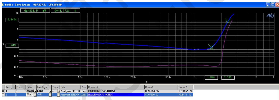
CST8002D (HL) THD VS PO 曲线 (5V 40HM 负载)
